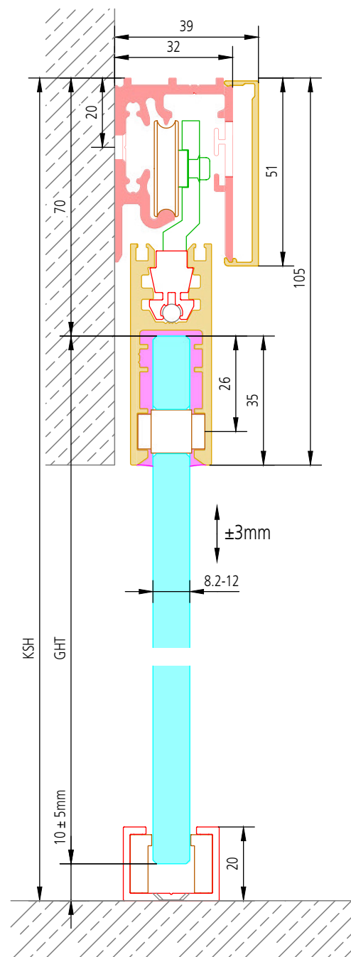
Wandmontage
